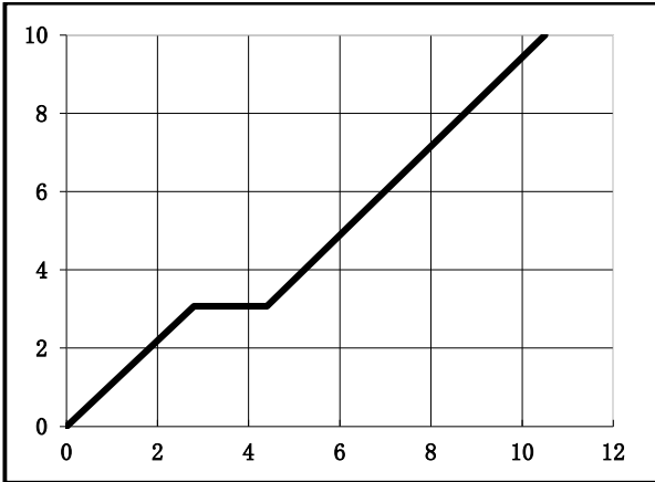
Fig.3 Power Dissipation Derating Curve
